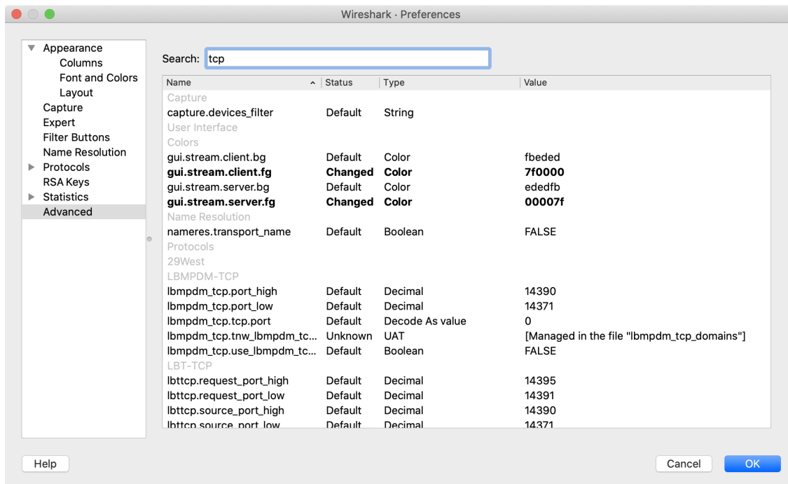
Figure 90. Advanced preferences
